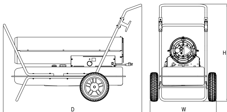
KFA125/170/210DGD Models
