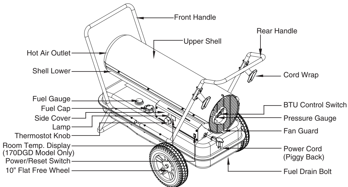
Figure 2. KFA125/170DGD MODELS
