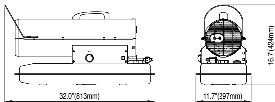
KFA50DGD/75DGD Models
