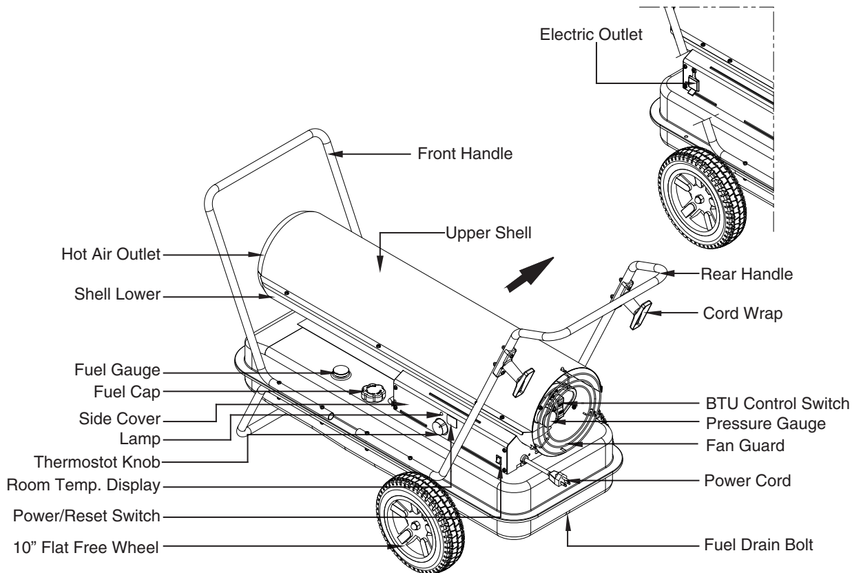
Figure 3. KFA210DGD MODEL
