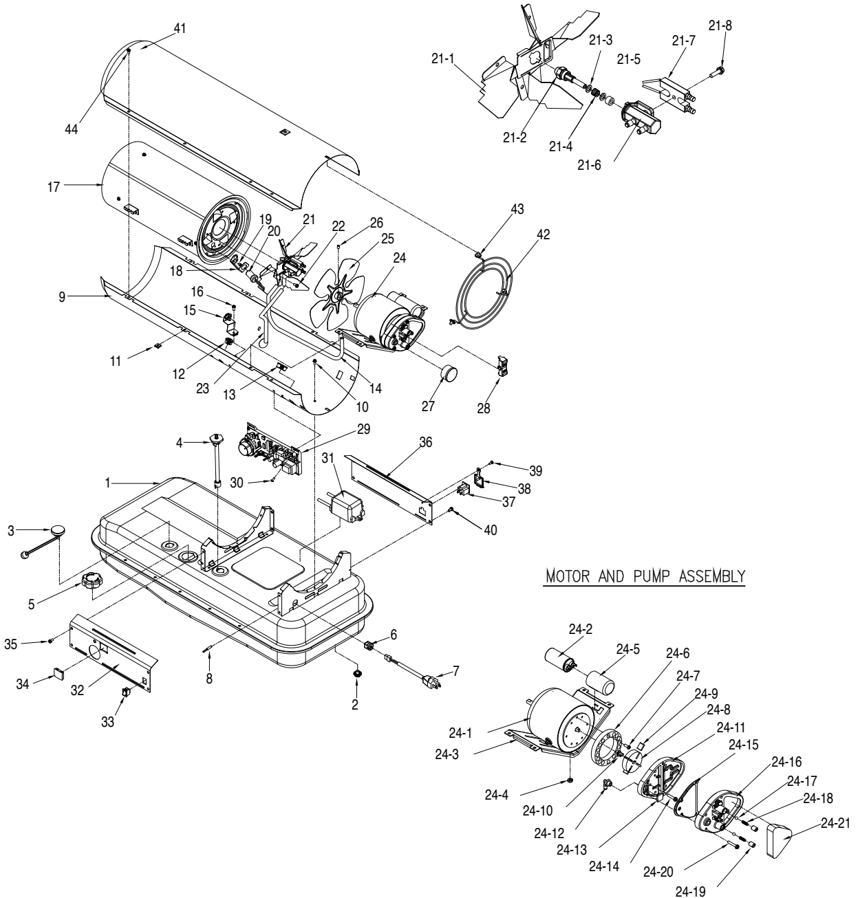
BURNER HEAD ASSEMBLY
