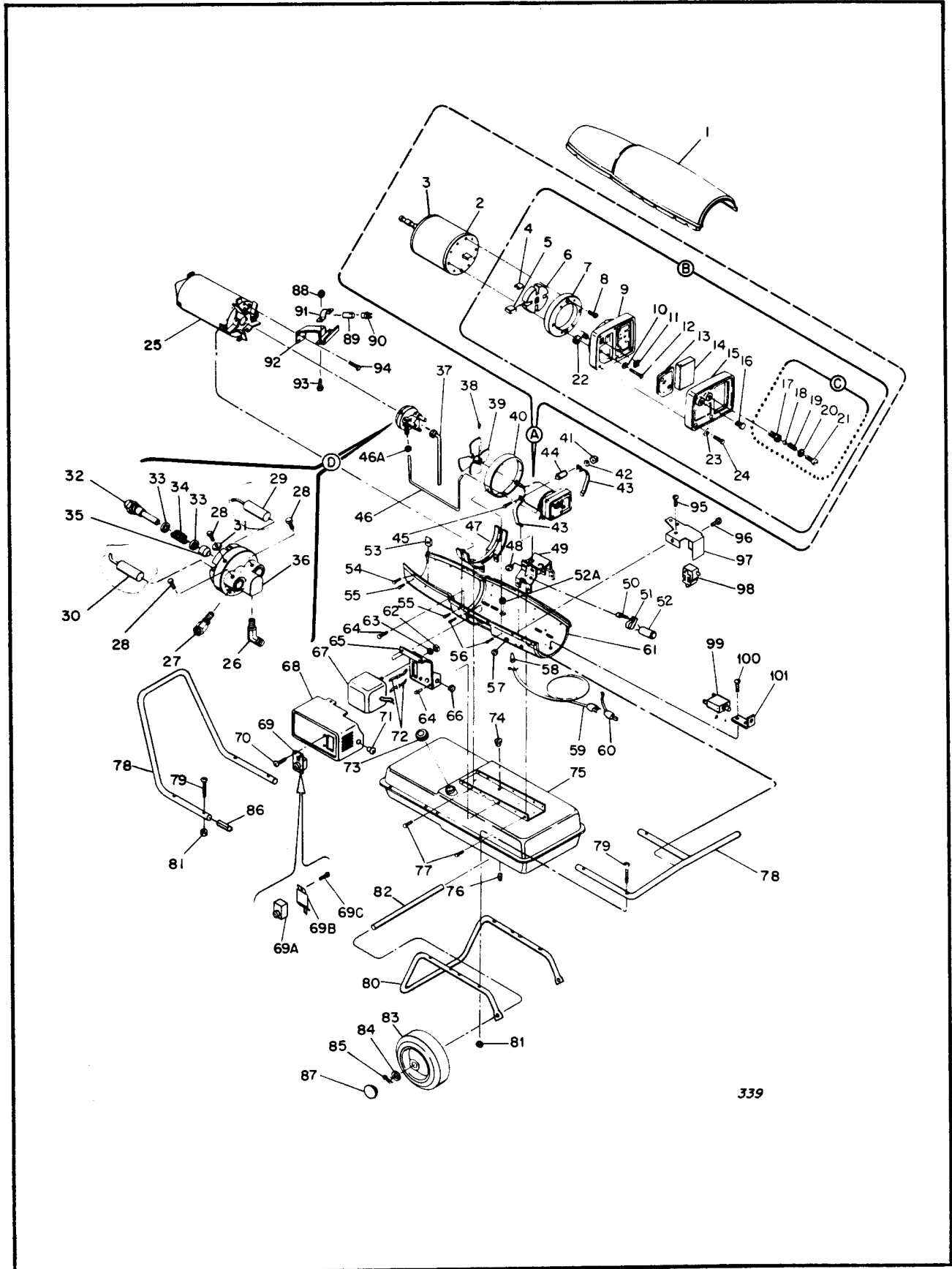
Figure 11. Mark 120 Deluxe Portable Heater; Exploded View
