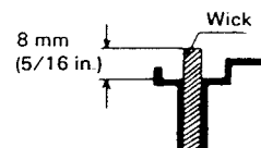
Wick Adjuster (Cutaway view)
